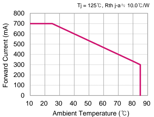
■ Derating Curve
